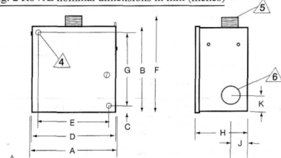
Fig. 2 R841E nominal dimensions in mm (inches)
